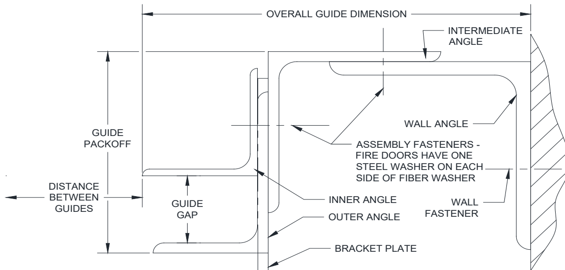
Figure 5.6 – Between Jambs Four-Angle Guide
