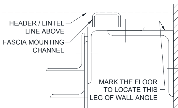
Figure 5.8 - Locating & Marking BJ Four Angle Guide Ass'y
