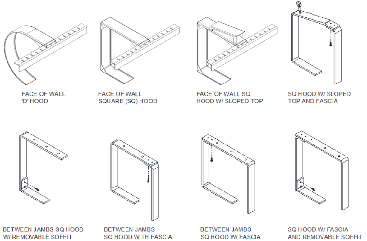
Figure 10.1 - Hood Supports
