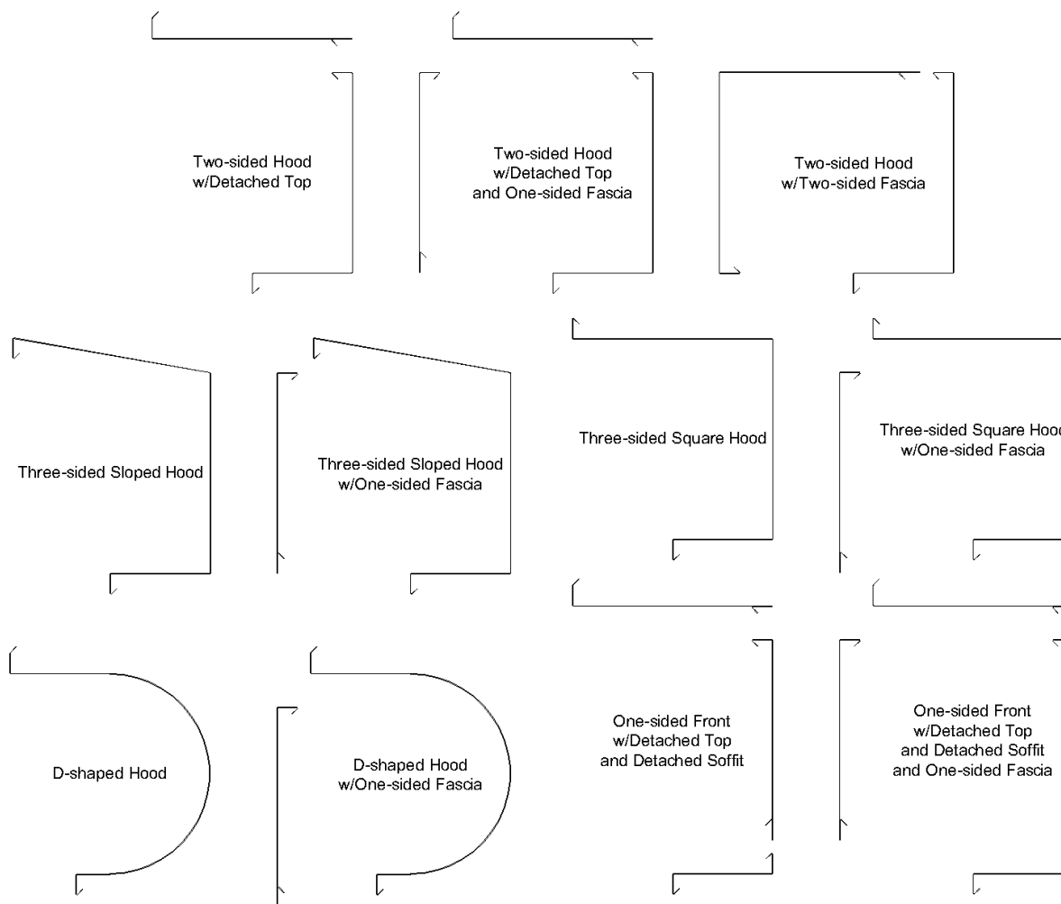
Figure 10.2 – Hood Configurations
