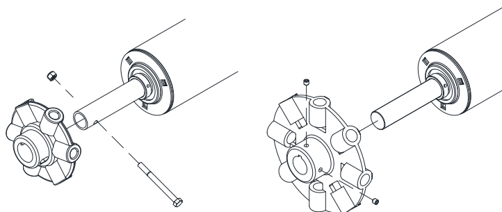
Figure 6.2 – Removal of adjustor from barrel assembly
