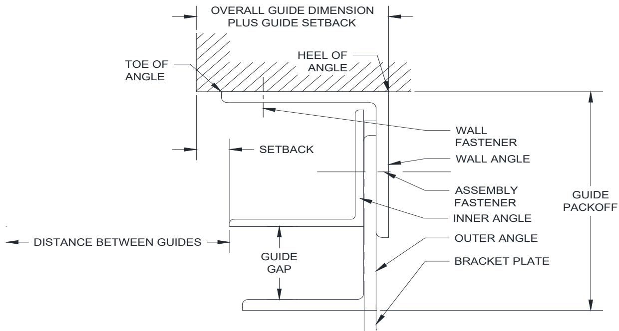
Figure 5.5 – Face of Wall “E” Guide with Windlock Flat
