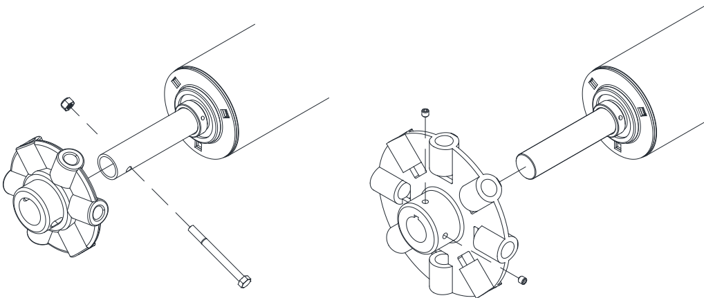
Figure 6.2 – Removal of Adjustor Wheel From Barrel Assembly
