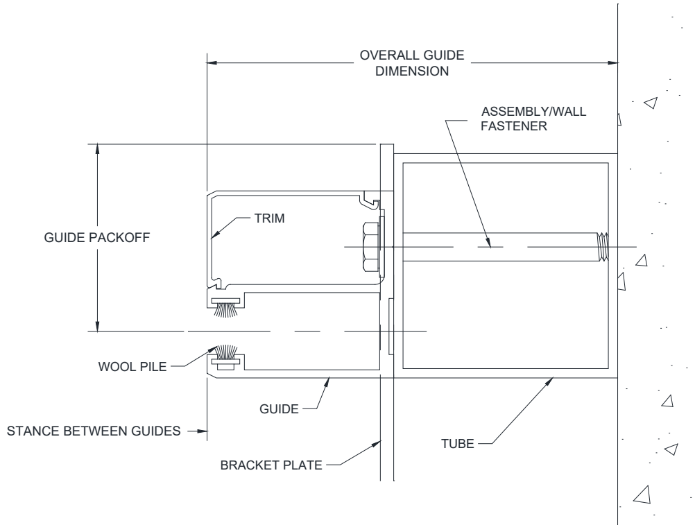
Figure 5.10 – Between Jambs with Tube Mounting to Wall
