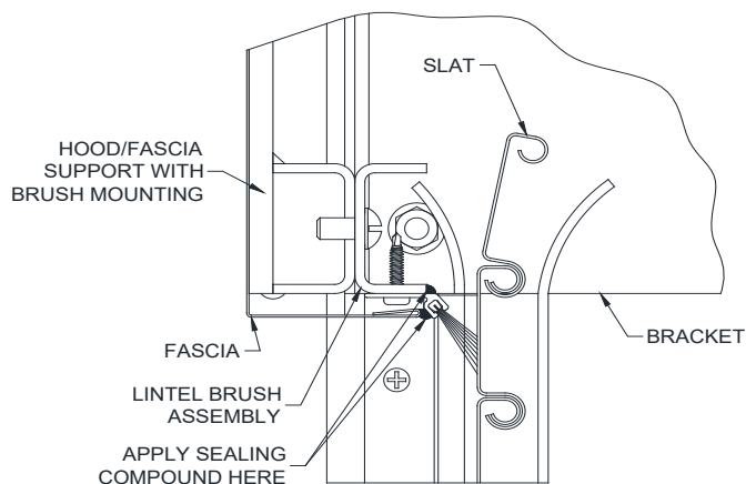
Figure 10.3 – Lintel Brush Channel Mounting to Guide
