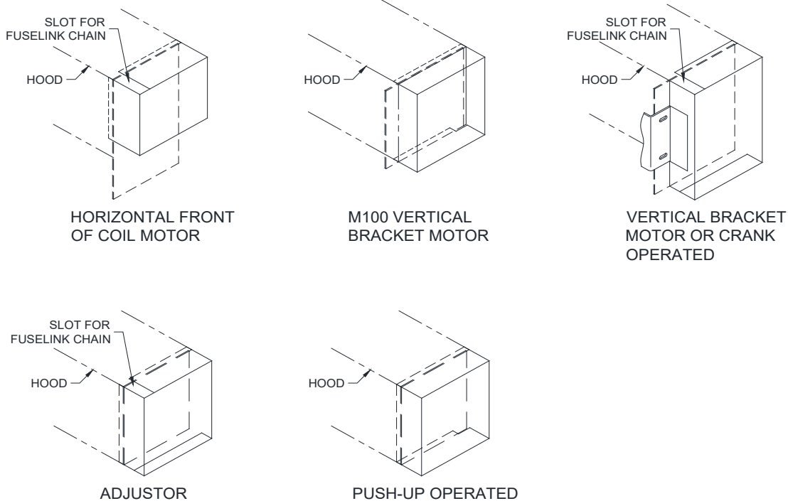
Figure 10.7 – Mechanism Covers
