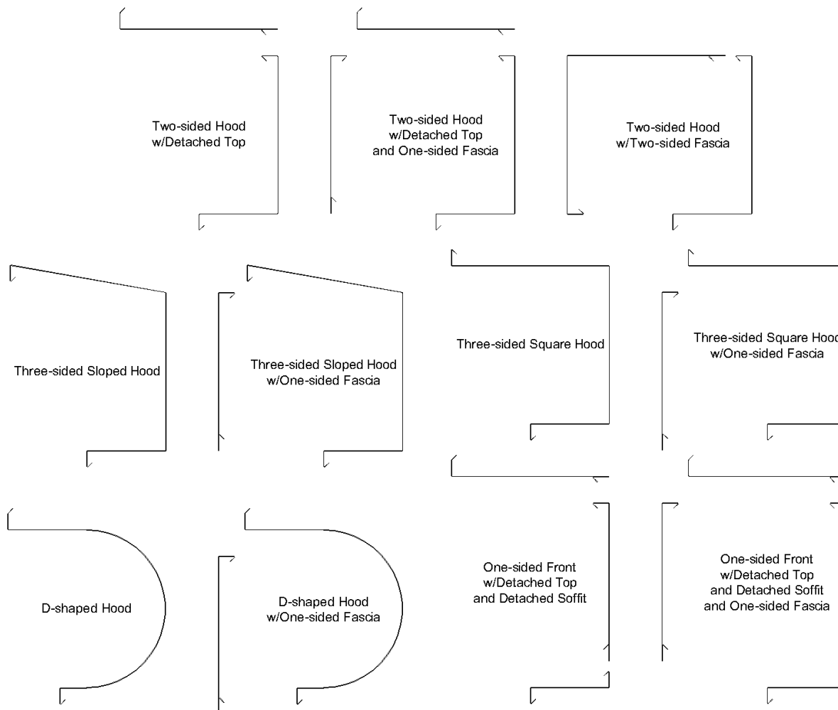
Figure 10.4 – Hood Configurations
