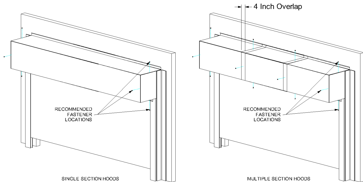
Figure 10.6 – Recommended Fastener Locations
