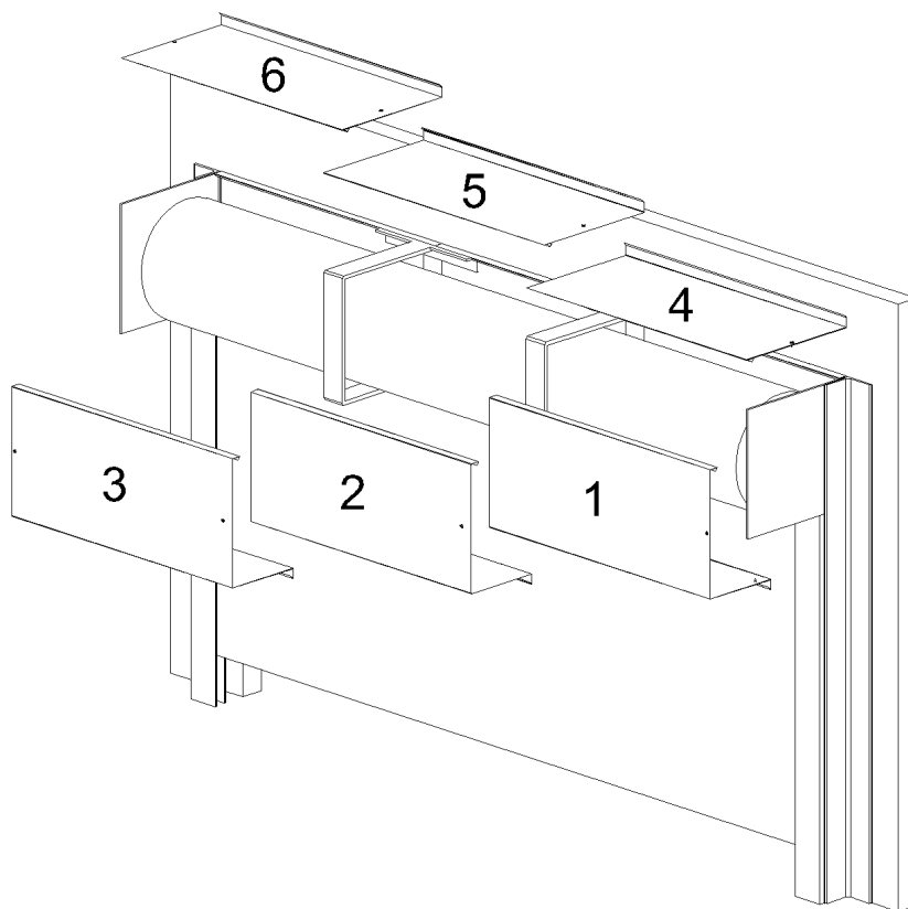
Figure 10.5 – Multiple Hood Sections
