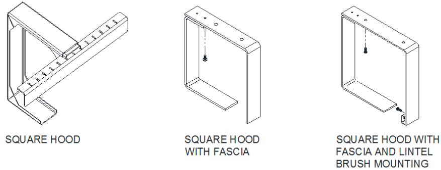
Figure 10.1 - Hood Supports
