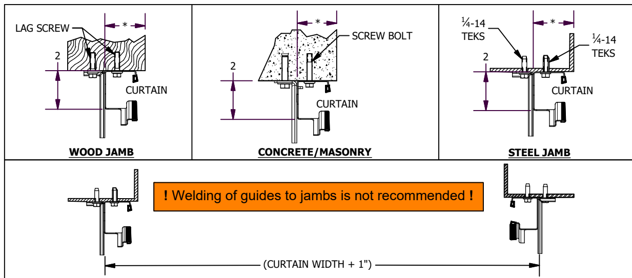
FIGURE 9: BACK OF GUIDE TO BACK OF GUIDE
