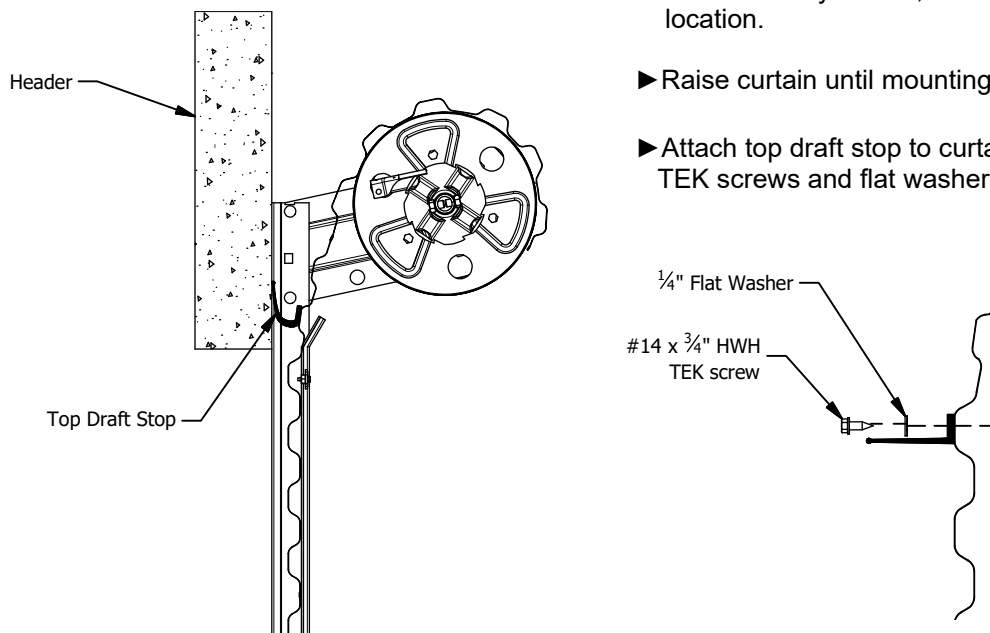
FIGURE 16: TOP DRAFT STOP INSTALLATION
