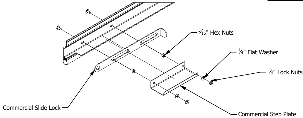
FIGURE 14: OPTIONAL BOTTOM BAR MOUNTED SLIDE LOCKS
