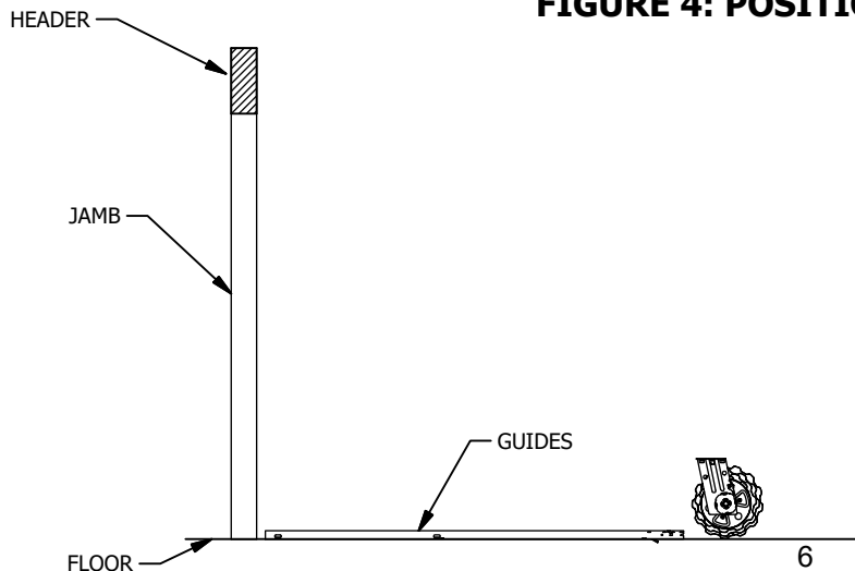
FIGURE 4: POSITION DOOR AND PARTS
