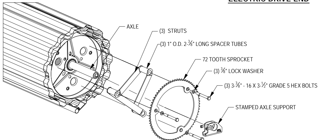
FIGURE 15: ELECTRIC DRIVE END
