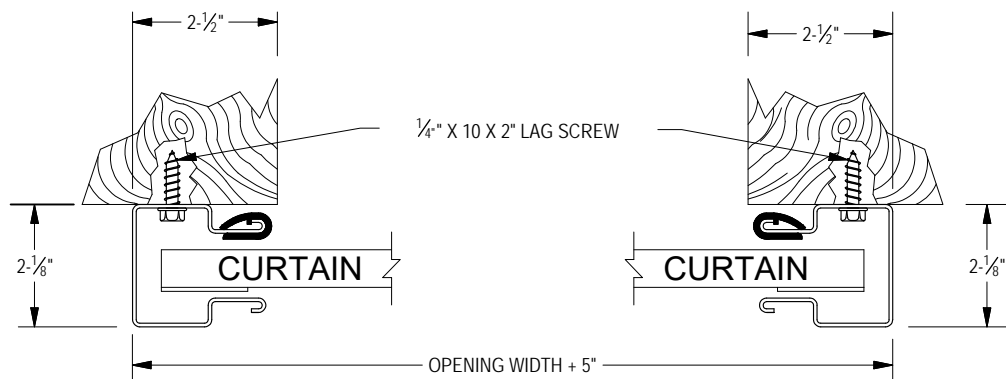
FIGURE 10: WOOD JAMBS
