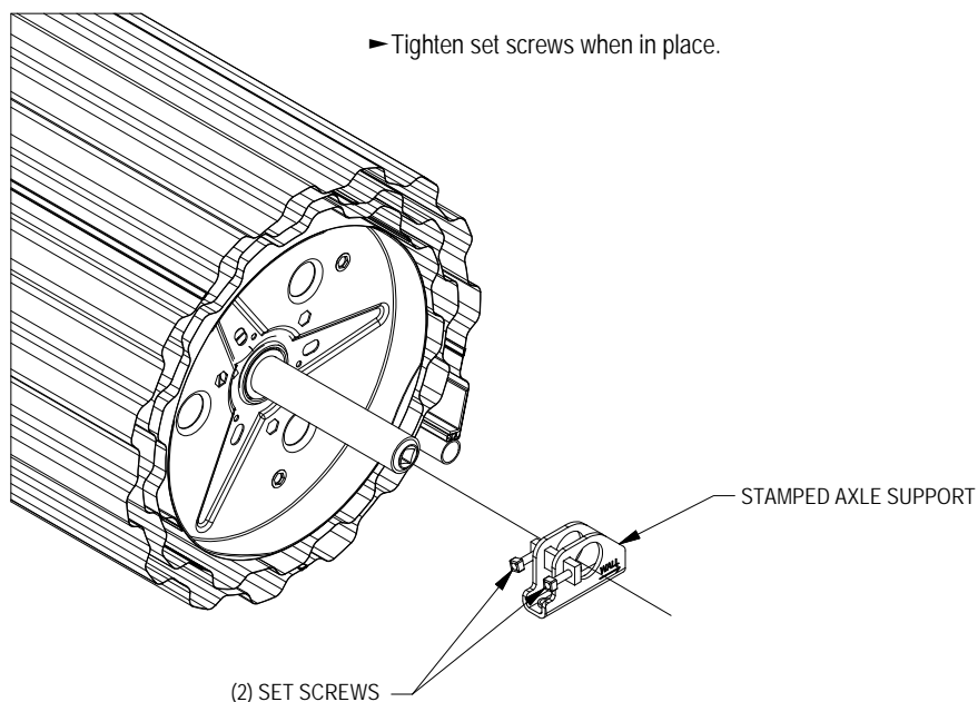
FIGURE 13: STAMPED AXLE SUPPORT END
