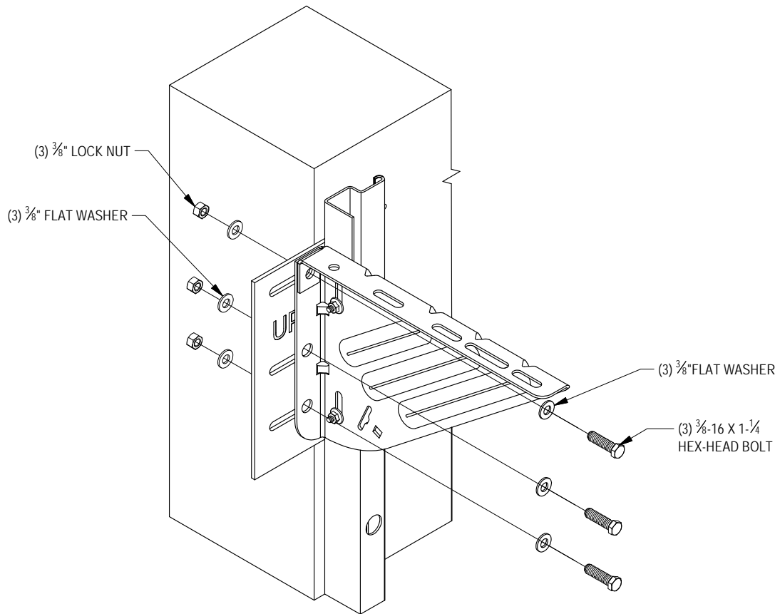
FIGURE 11: BRACKETS MOUNT TO STEEL JAMBS VIA MOUNTING PLATES
