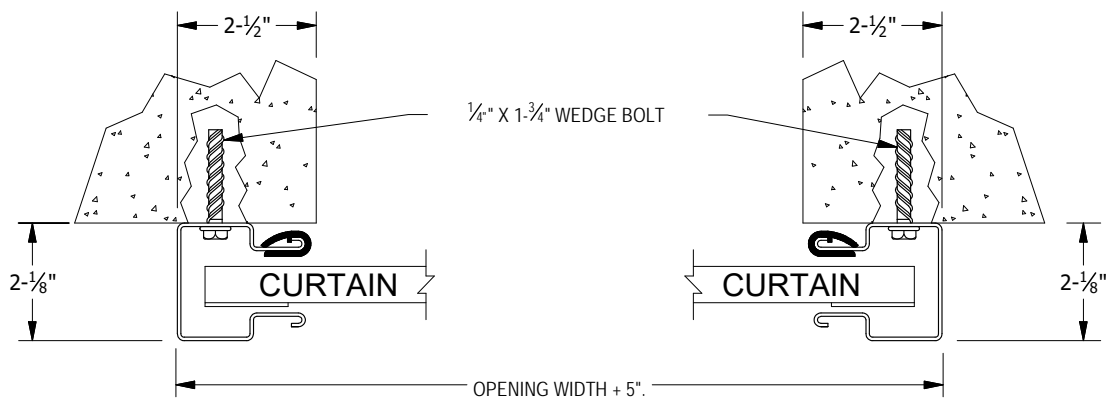
FIGURE 9: CONCRETE / MASONRY JAMBS
