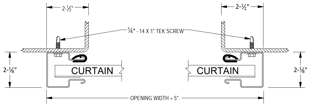
FIGURE 8: STEEL JAMBS
