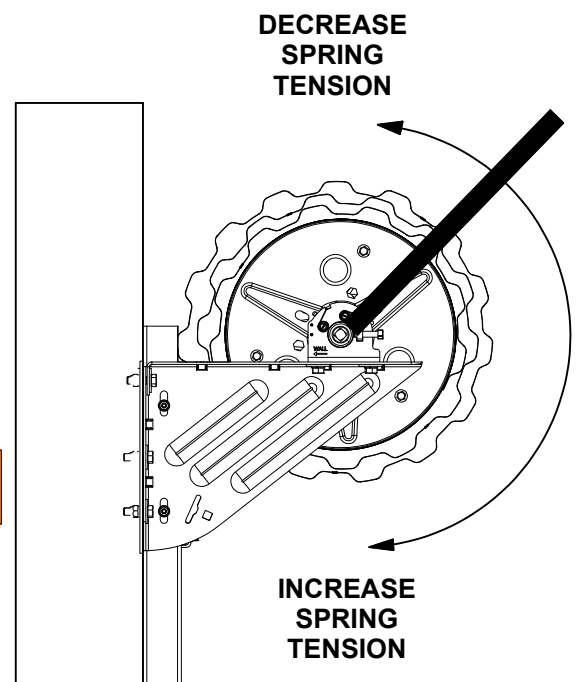
FIGURE 23: ADJUST SPRING TENSION
